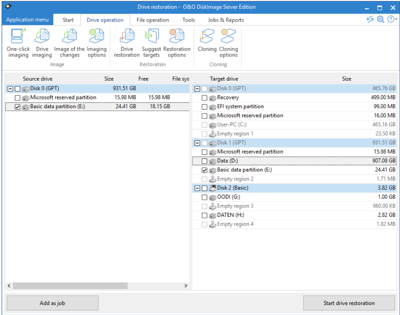
Restore drives
