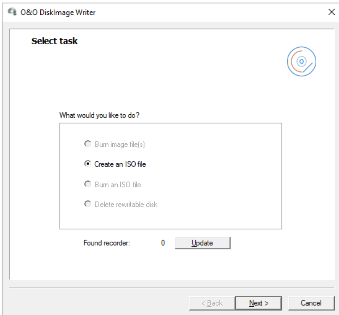
Burn Wizard
